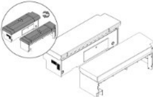
3. Flip the cushions and swap them on each bunk.
