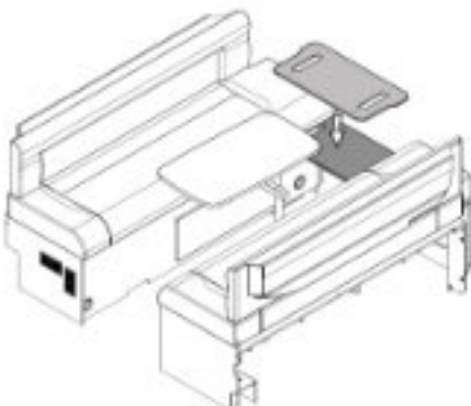
1. Insert the panel into the clips located on the edge of each bunk.
