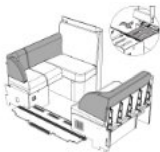
1. Remove and store the backrests highlighted. Make sure to unfold the support for the centre piece.
