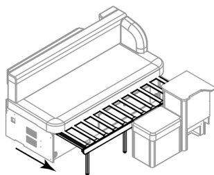
3. Pull out the bunk support from under the bunk so that it is fully extended.
