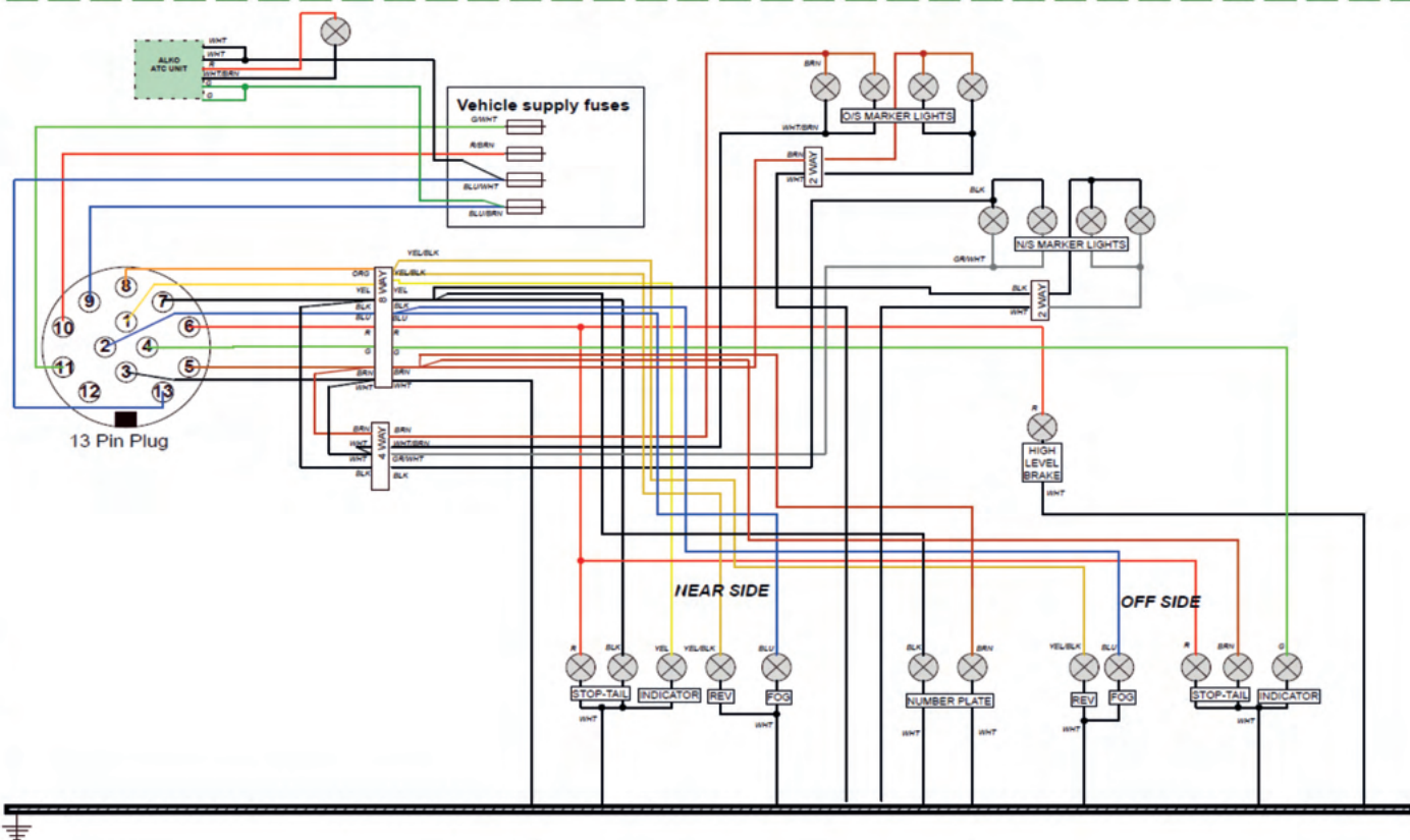
Discovery, Phoenix Black Edition & Pegasus Black Edition - Road Light System
