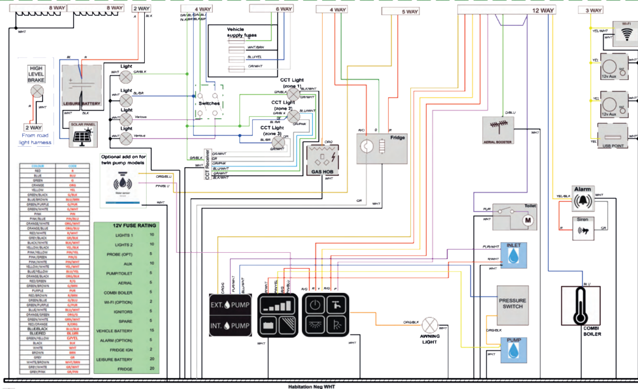
Unicorn Deluxe Twin Axle - Electrical System
