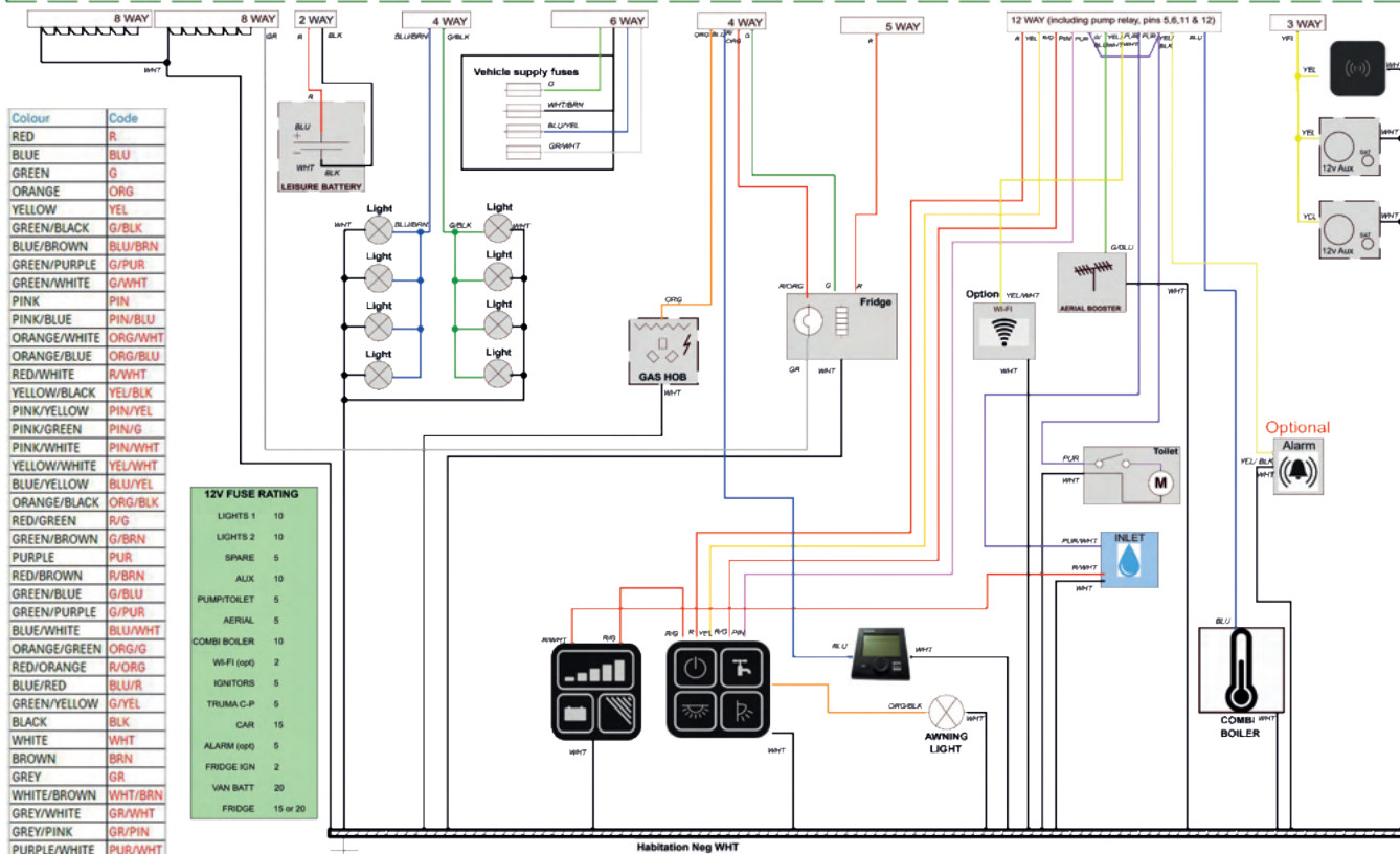
Phoenix Black Edition All Models - Electrical System
