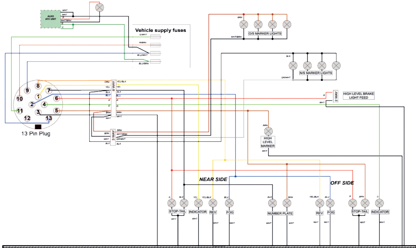
Alicanto Grande Deluxe & Unicorn Deluxe - Road Light System
