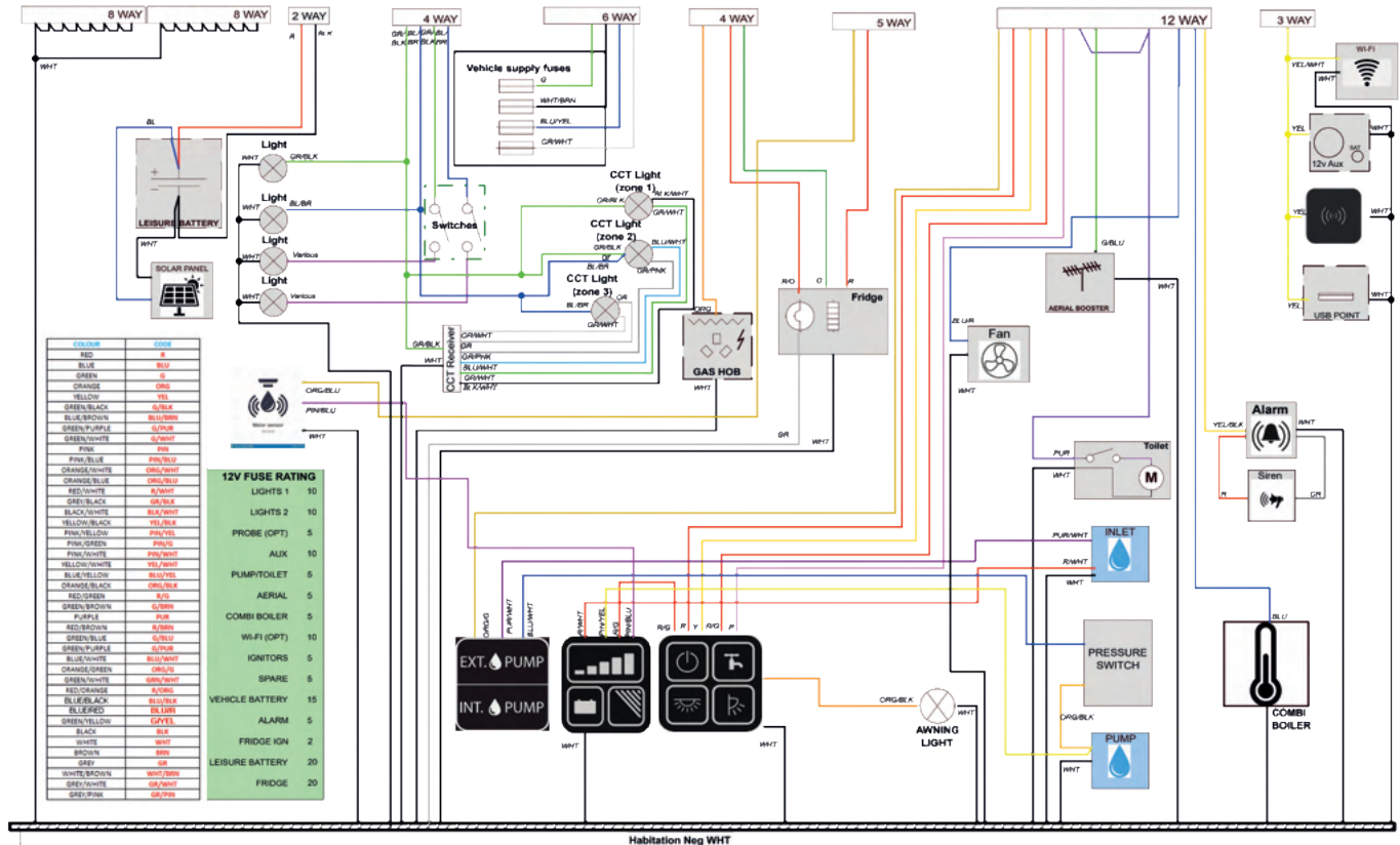
Alicanto Grande Deluxe Twin Wht Axle - Electrical System
