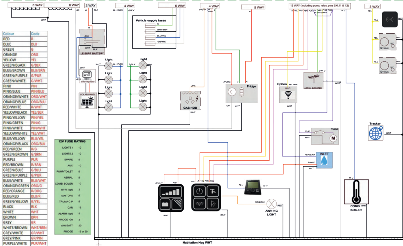
Pegasus Black Edition All Models - Electrical System
